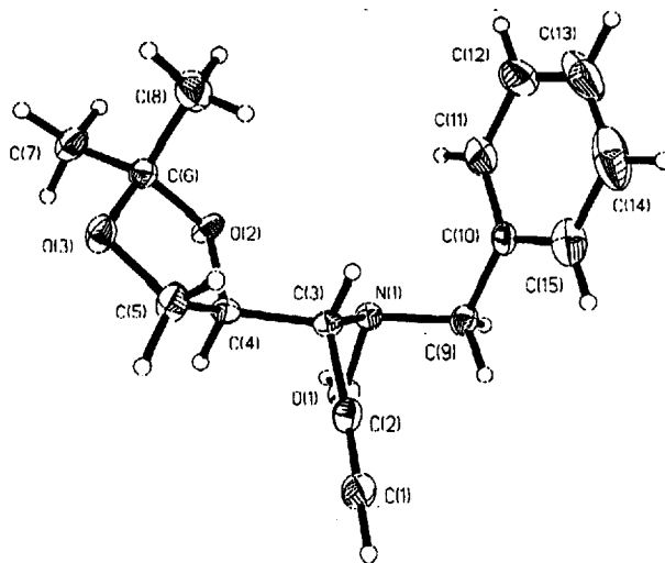
Figure 1. ORTEP view of compound 5 showing ellipsoids at a 30% probability level.
